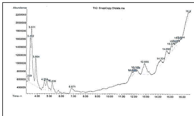
Figure 1. GC-MS Chromatogram of WGO
